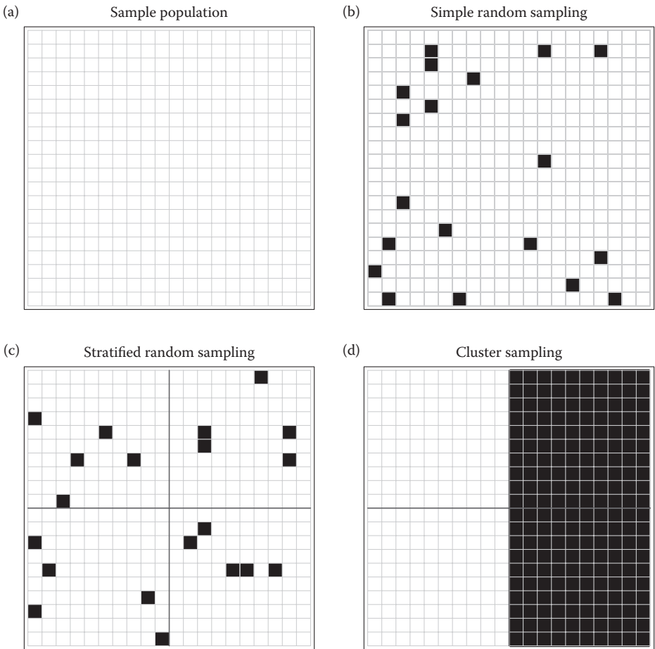
FIGURE 7.3 Demonstration of sampling designs. (a) An entire population of 400 experimental units (i.e., elements in a 20 \times 20 grid). (b) A simple random sample of 20 from the population. (c) A stratified random sample; four strata are established and five samples are randomly taken from within each strata. (d) Cluster sampling; four clusters are established, two of these are randomly selected and a census is taken from each selected cluster.
