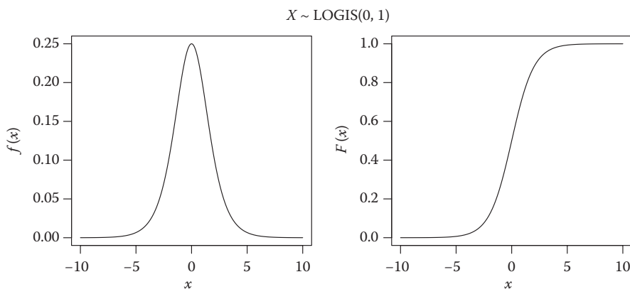
FIGURE 3.27 The pdf and cdf for \text{LOGIS}(0, 1) .
